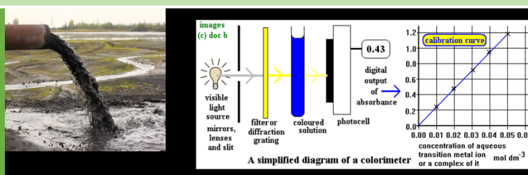
Colorimeter based optical sensor device is being developed for heavy metal detection in water
